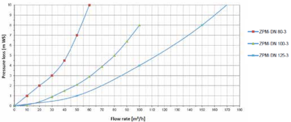
Pressure loss DN 80 - DN 125
