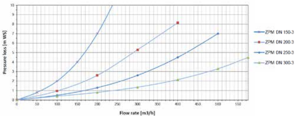
Pressure loss DN 150 - DN 300
