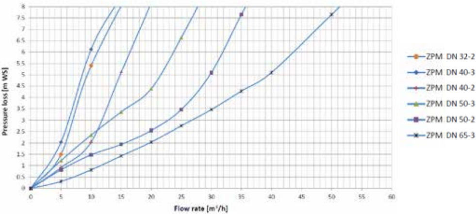
Pressure loss DN 32 - DN 65
