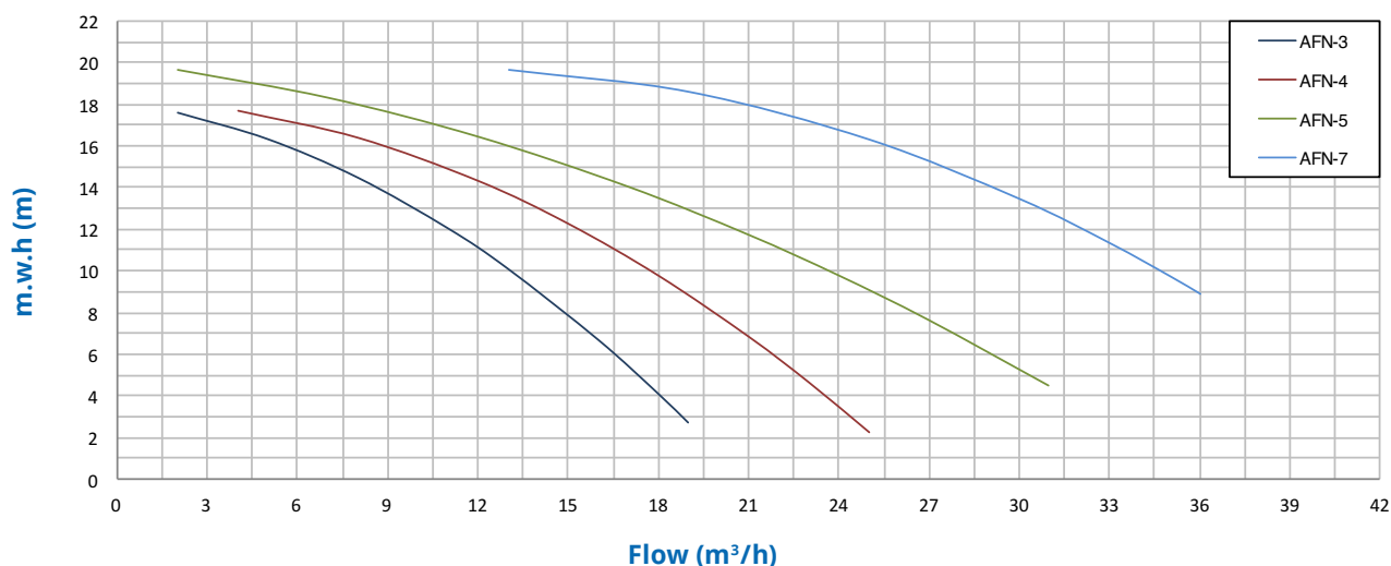
Characteristics curve
