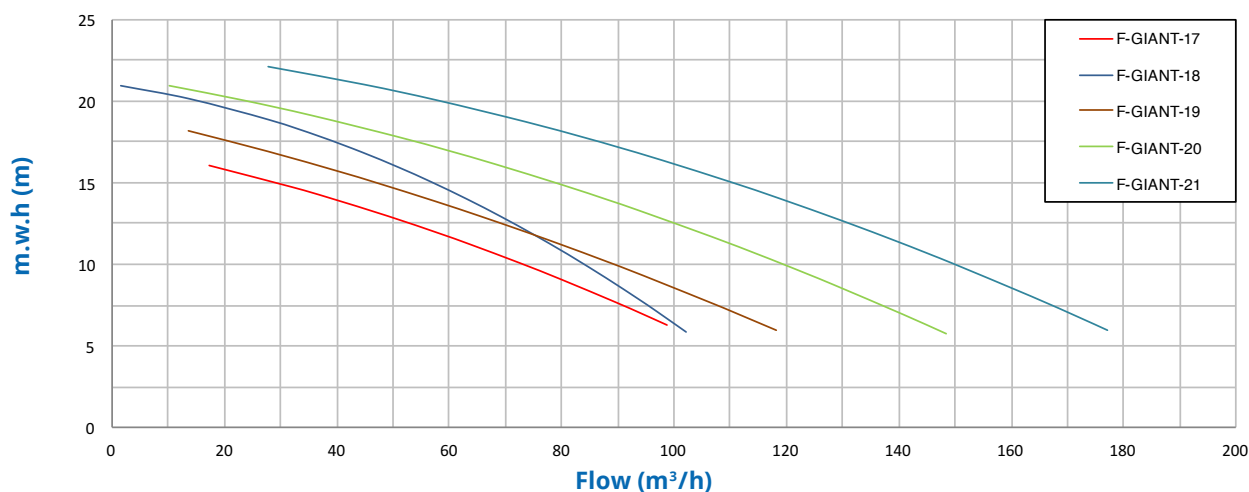
Characteristics curve
