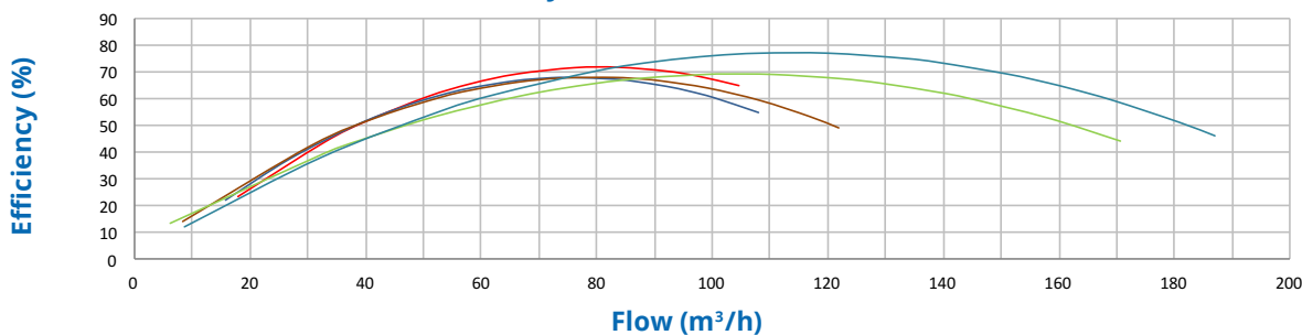
Hydraulic Performance
