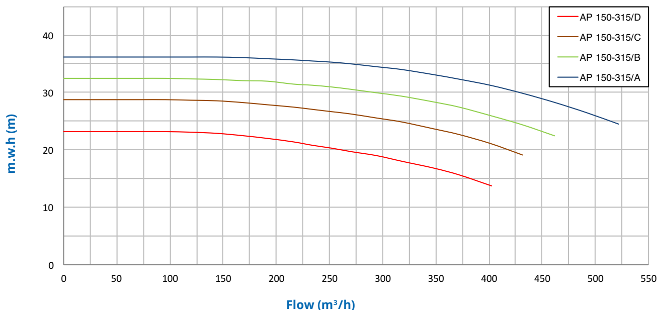
Characteristics curve
