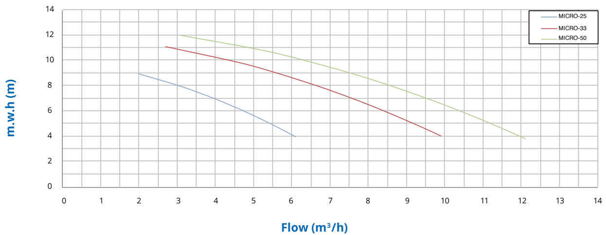
Characteristics curve
