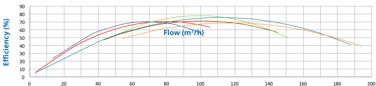
Hydraulic Performance
