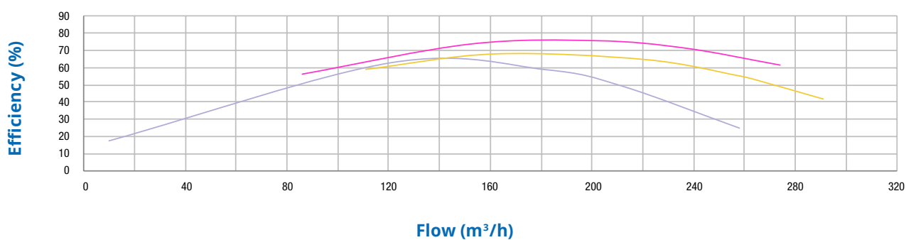
Hydraulic Performance
