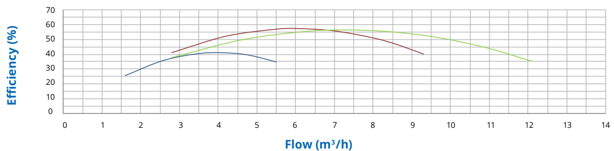
Hydraulic Performance
