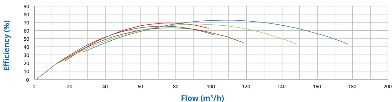
Hydraulic Performance
