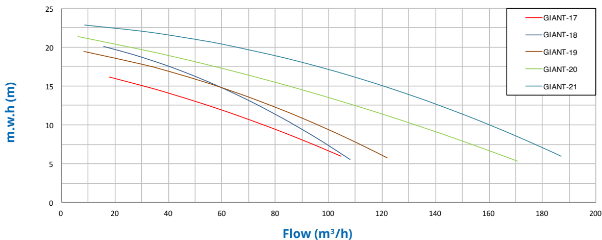
Hydraulic Performance
