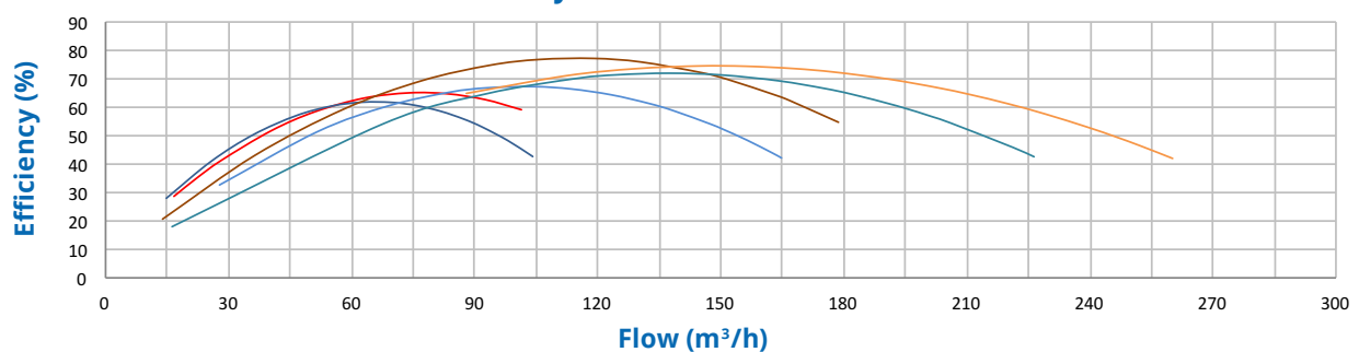
Hydraulic Performance
