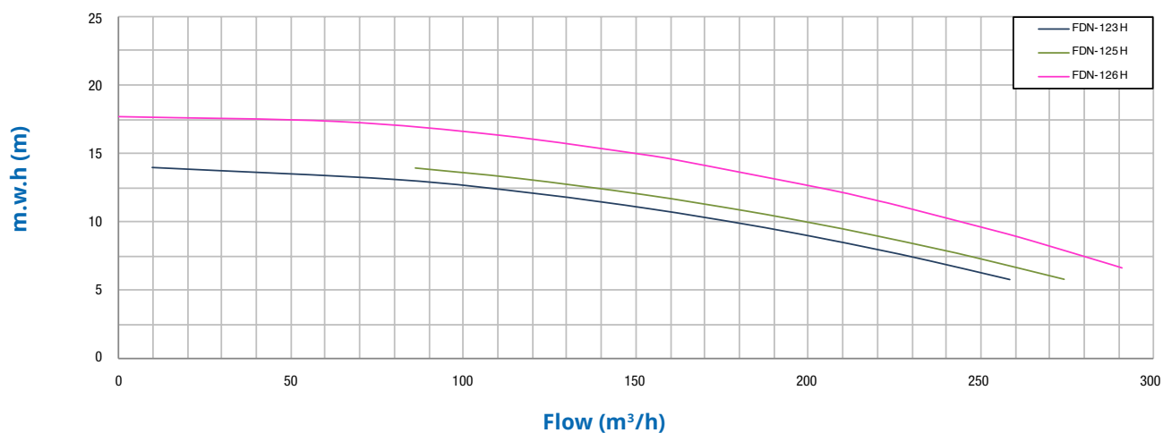
Characteristics curve
