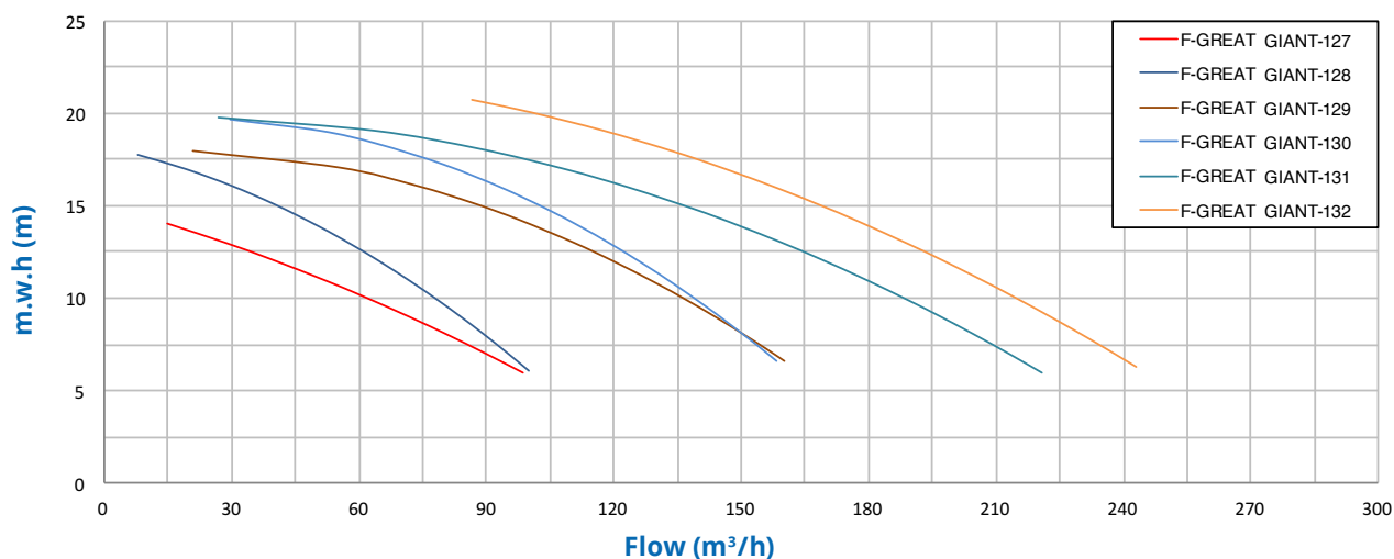
Characteristics curve
