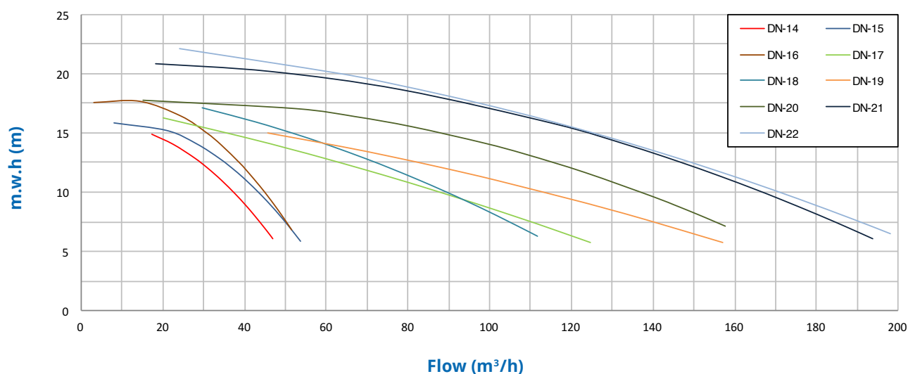
Characteristics curve
