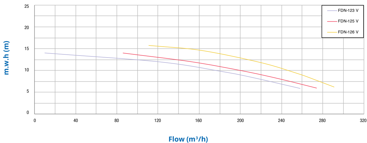
Characteristics curve
