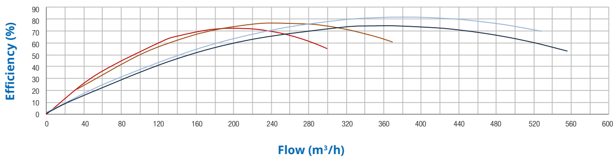
Hydraulic Performance
