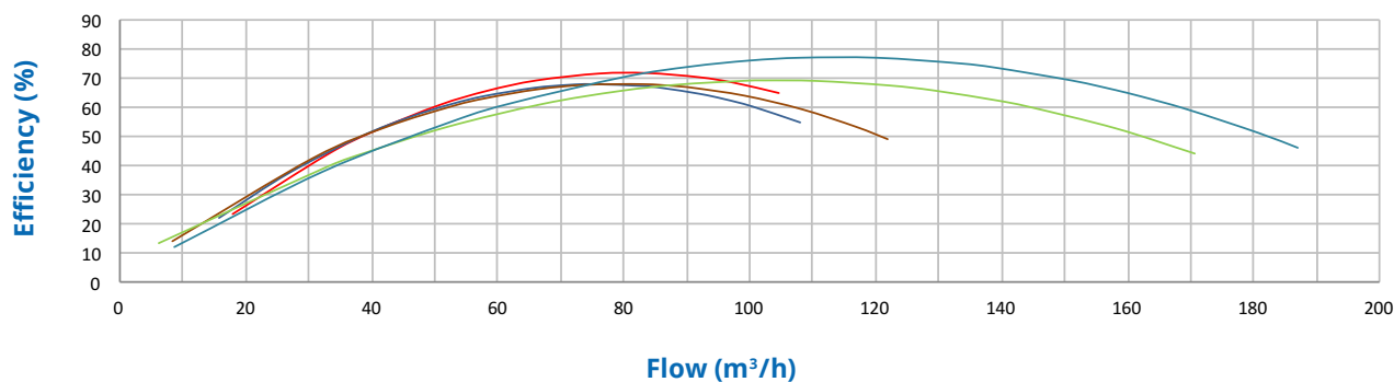
Hydraulic Performance
