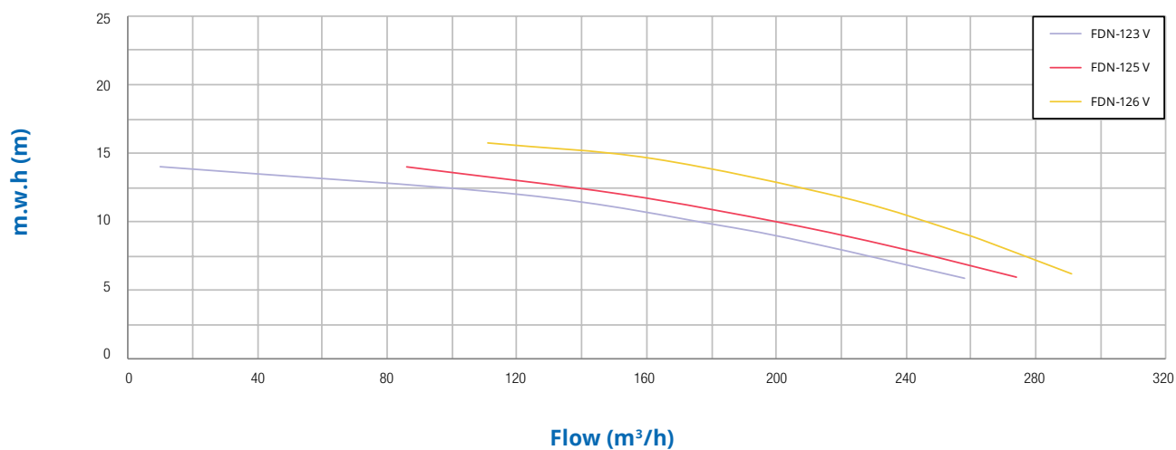
Characteristics curve
