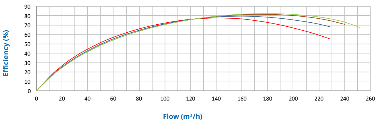
Hydraulic Performance
