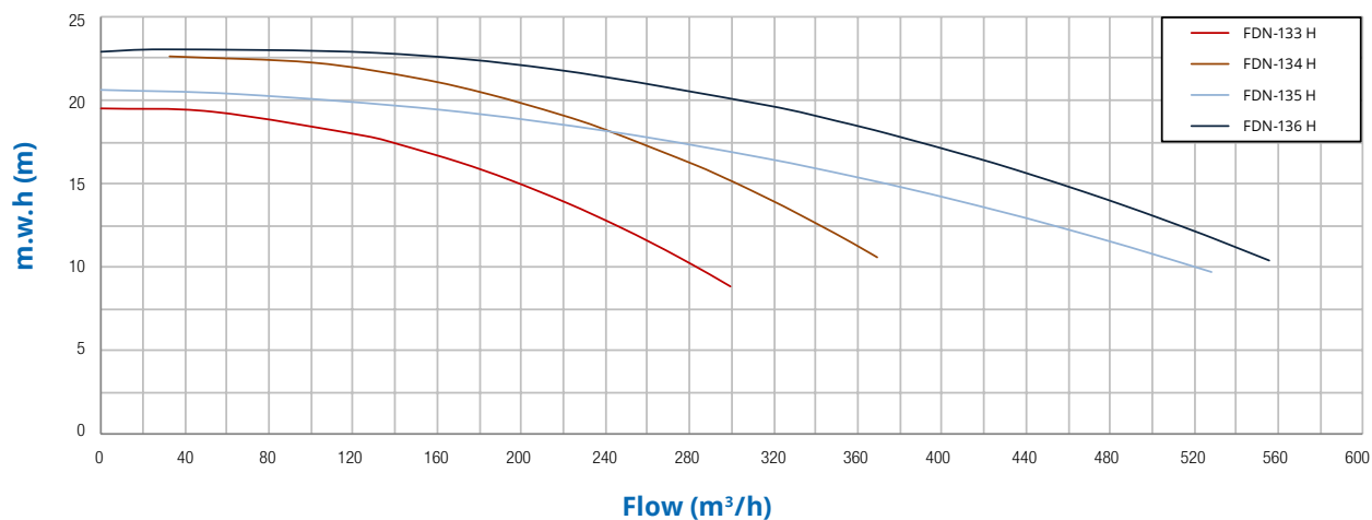
Characteristics curve
