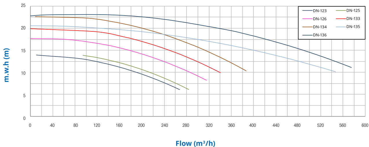
Characteristics curve
