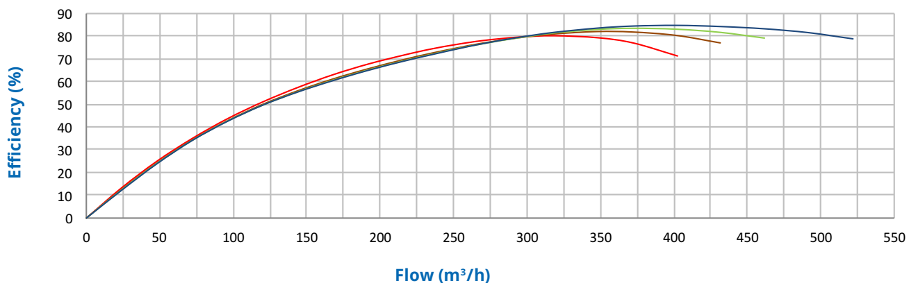
Hydraulic Performance
