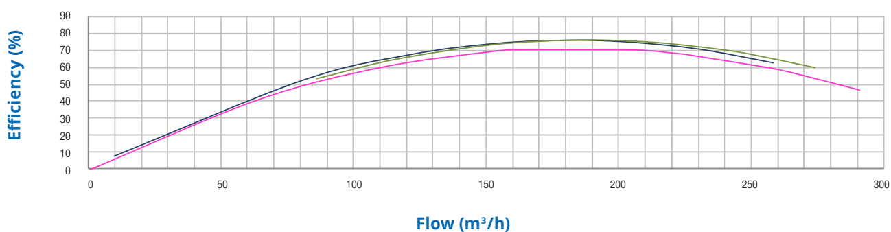
Hydraulic Performance
