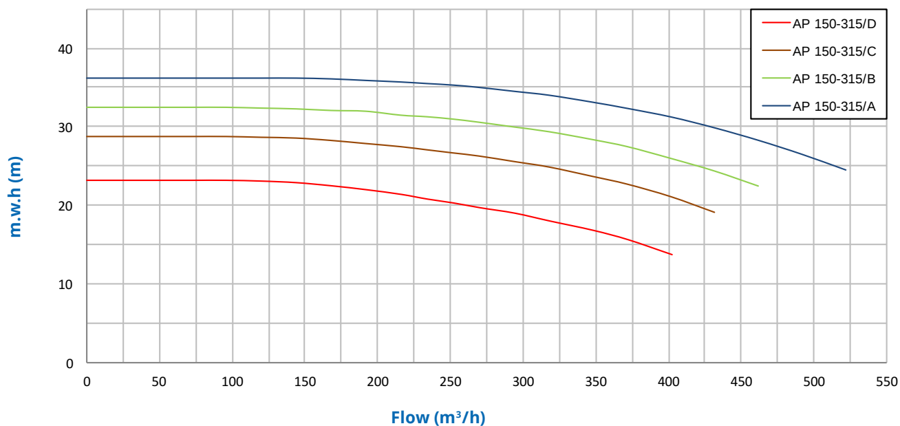
Characteristics curve
