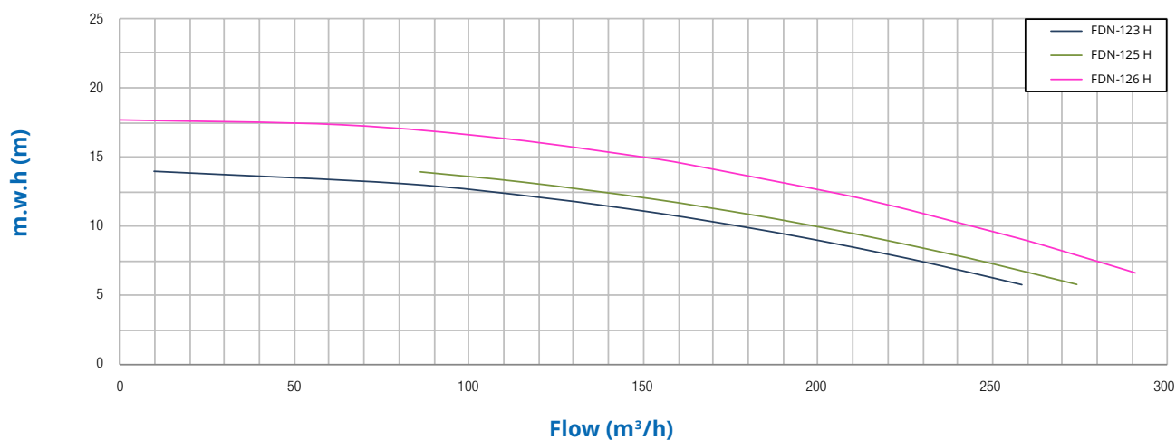
Characteristics curve
