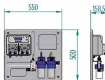
HPP TWIN pH/REG
