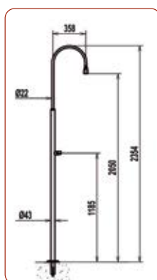
Grifo manual Manual tap
