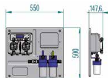
HPE TWIN FCLINORG
