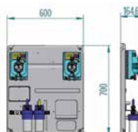
HPE TOP pH-ORP
